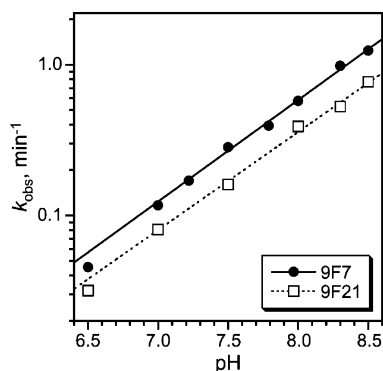
FIGURE 3: pH dependence of the ligation rate k_{\text{obs}} for 9F7 and 9F21. Assays were performed in 50 mM buffer, 150 mM NaCl, 2 mM KCl, and 20 mM \text{MnCl}_2 at 37 °C. The buffer compound was PIPES (pH 6.5), HEPES (pH 7.0–7.8), or EPPS (pH 8.0–8.5). Data acquired at higher pH (8.8–9.0 with CHES) were discarded due to obvious \text{Mn}^{2+} oxidation (development of brown color in the reaction solution). The fit lines have slopes of 0.71 (9F7) and 0.68 (9F21). The left-hand substrate was ...UA↓(uc) prepared by solid-phase synthesis.
