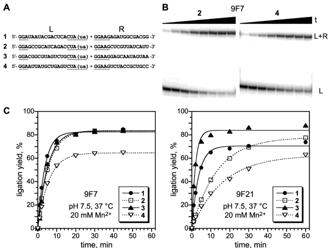
FIGURE 6: Survey of the ligation activities of 9F7 and 9F21 with RNA substrate sequences that vary away from the ligation site. (A) The four RNA substrate combinations, 1–4. Nucleotides that are constant among all four sequences are underlined (the 5'-GGA is to permit transcription; the nucleotides nearer the ligation junction are investigated in Figures 4 and 5). As may be verified by looking vertically down each column of nonunderlined nucleotides, each of the four nucleotides, U, C, A, and G, is represented at every position in one of the four substrate combinations, 1–4. For all RNA nucleotides within the substrate binding arms (see Figure 1B), the corresponding DNA nucleotide was the Watson–Crick complement, except in the 9F7 left-hand DNA binding arm, where one nucleotide was intentionally deleted as described in Figure 11. The left-hand substrates were prepared by transcription terminating with a 2',3'-cyclic phosphate. (B) Representative PAGE images for substrates 2 and 4 assayed with 9F7. For a gel image for 1, see Figure 1C, but note that the left-hand substrate in that figure has a different 3'-terminal nucleotide (C with a 2',3'-diol in Figure 1C instead of A with a 2',3'-cyclic phosphate here), so the k_{\text{obs}} values are not identical. (C) Kinetic plots for all four substrate combinations for 9F7 (left) and 9F21 (right). k_{\text{obs}} values for 9F7: 1, 0.27 min -1 ; 2, 0.18 min -1 ; 3, 0.19 min -1 ; 4, 0.17 min -1 . k_{\text{obs}} values for 9F21: 1, 0.28 min -1 ; 2, 0.075 min -1 ; 3, 0.53 min -1 ; 4, 0.061 min -1 .
